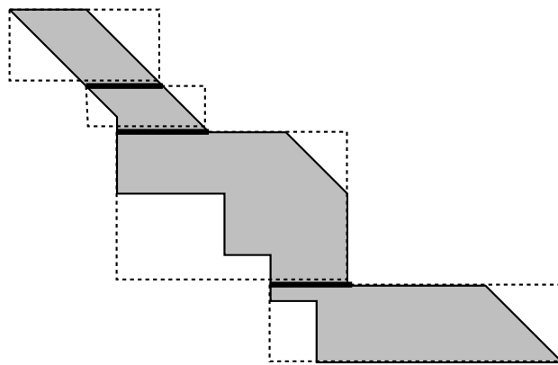
FIG. 10. Covering a narrow region, R , with non-intersecting rectangles, each of which has more points in R than outside R . The dark lines show where values of S^+ are saved during the backward pass described in the text.
